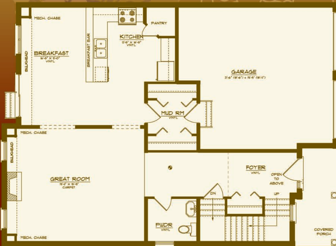
Main Floor 1,060 Sq. Ft.
